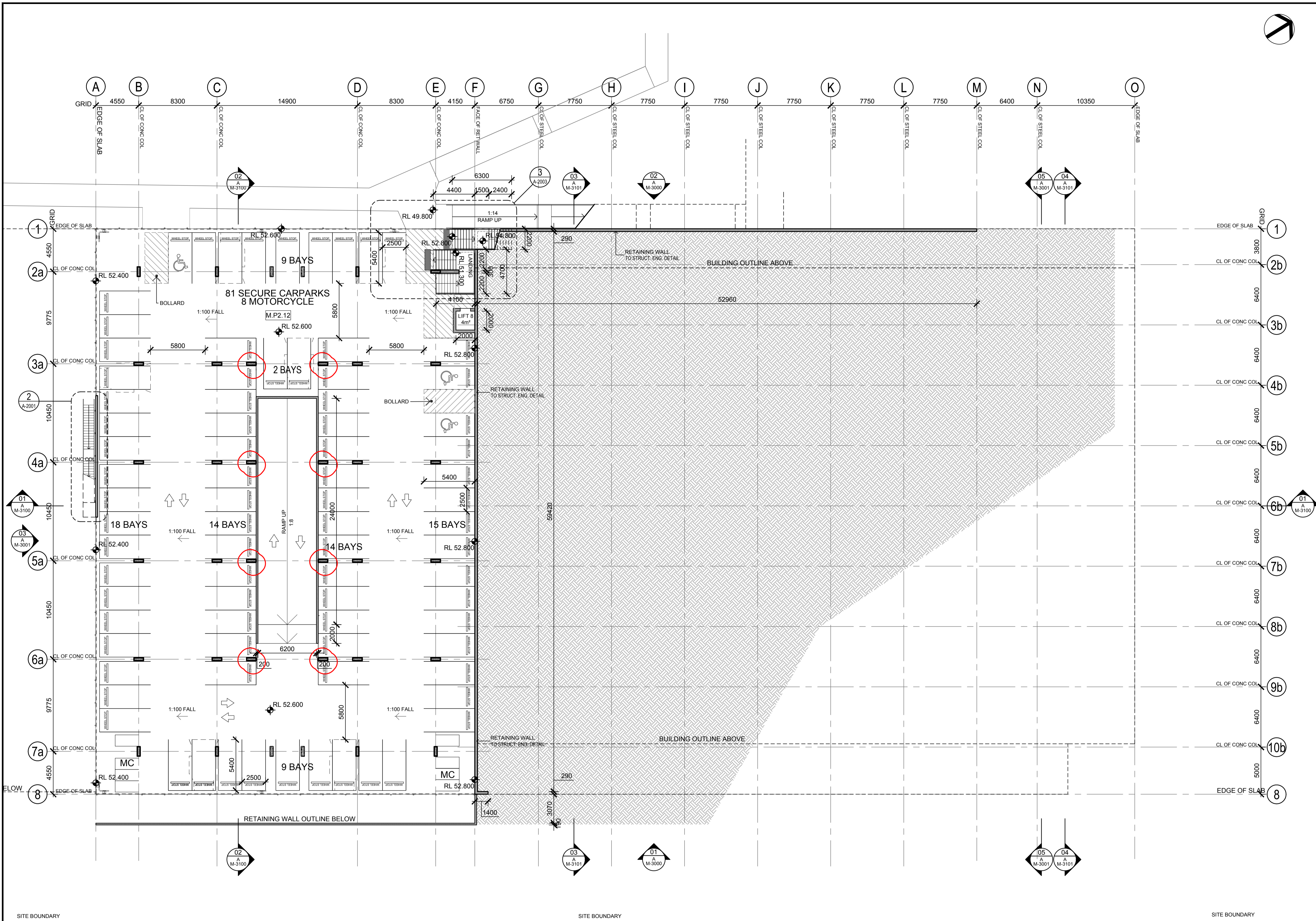
PARKING P2 PLAN SCALE 1:200 @ A1
